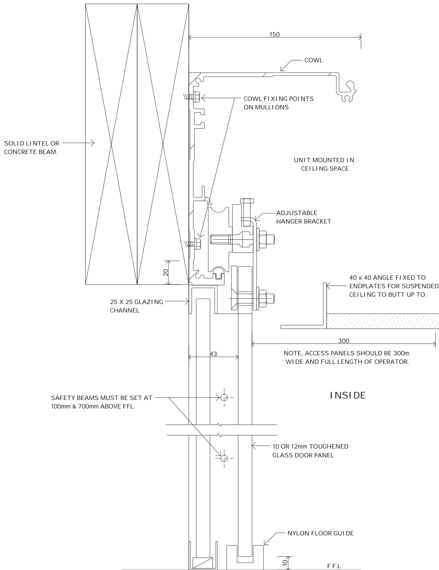
TYPICAL VERTICAL SECTION AT FRAMELESS DOORS MOUNTED IN CEILING SCALE 1:2
